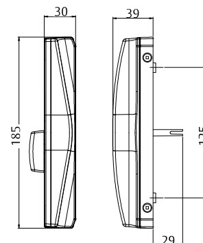
Snib & Cylinder
